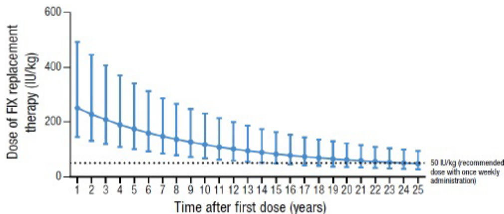
Figure 5-3: Median (90% PI) dose of FIX replacement therapy (eftrenonacog alfa; once weekly fixed frequency) required to maintain trough FIX activity at the time-matched mean fidanacogene elaparvovec response (picture taken from [40])
