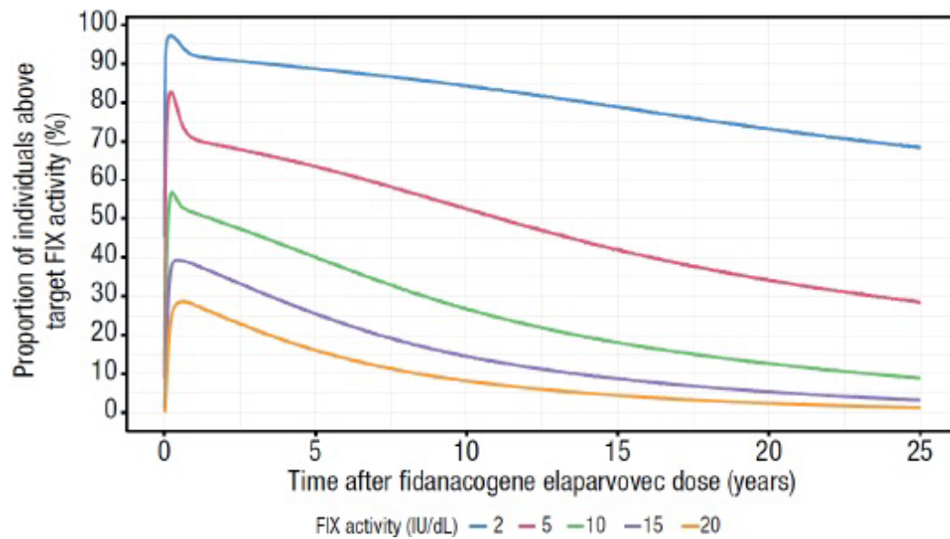
Figure 5-2: Proportion of individuals in the simulated population with predicted FIX activity above the selected target levels. FIX = factor IX (picture taken from [40])
